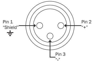
XLR Output Connector Assignment of SR40/HC
