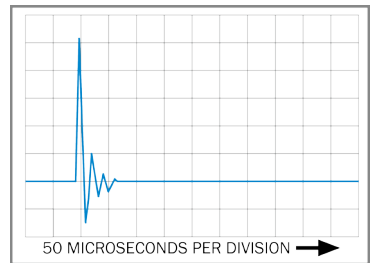
Impulse Response of SR40/HC (typical)
