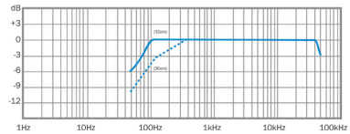
Frequency Response of SR40/HC (typical)
